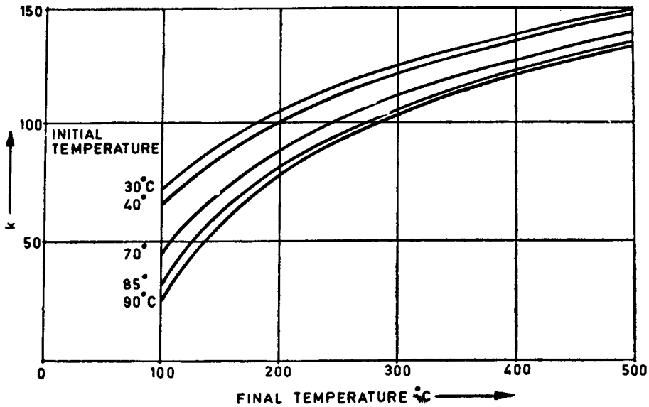
FIG. 19 k FACTORS FOR ALUMINIUM PROTECTIVE CONDUCTORS
