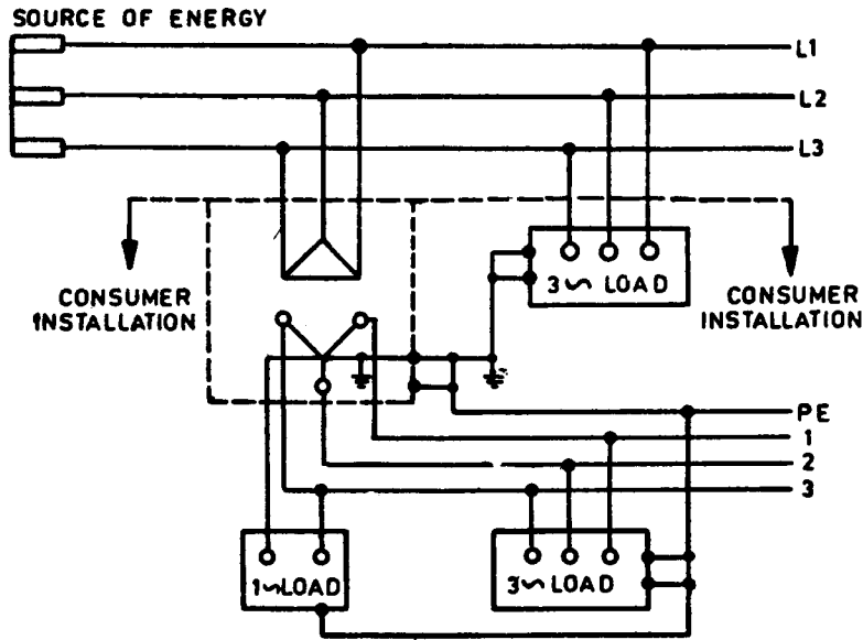
6.6/11 kV Three phase bulk supply.
