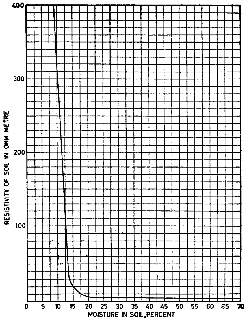
FIG. 9 VARIATION OF SOIL RESISTIVITY WITH MOISTURE CONTENT
