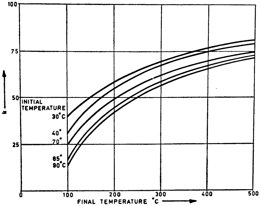
FIG. 18 k FACTORS FOR STEEL PROTECTIVE CONDUCTORS
