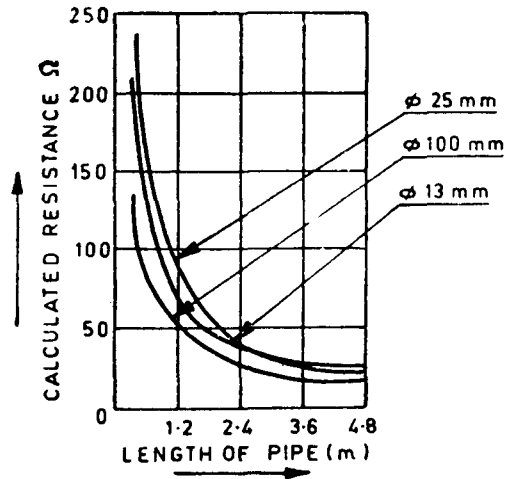
FIG. 11 EFFECT OF LENGTH OF PIPE ELECTRODE ON CALCULATED RESISTANCE FOR SOIL RESISTIVITY OF 100 \Omega \cdot \text{m} ( ASSUMED UNIFORM )
