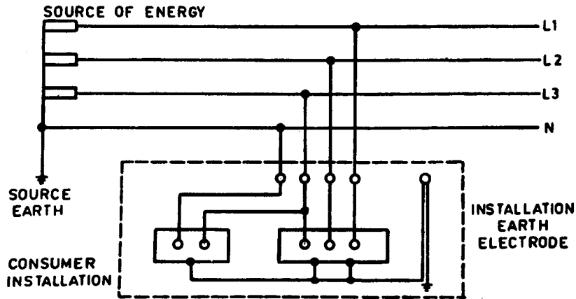
415 V Three phase industrial supply having 3 ~ and 1 ~ loads.
