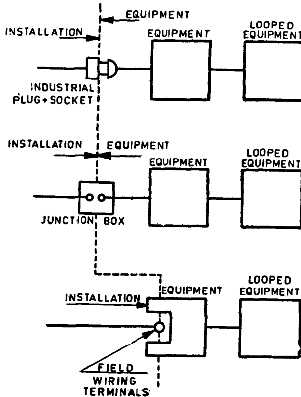
FIG. 37 EQUIPMENT-INSTALLATION BOUNDARIES
